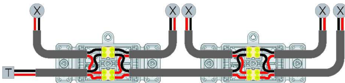
Schema di collegamento in parallelo Wiring diagram parallel connections
