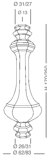
E014 \varnothing 83 x H250
