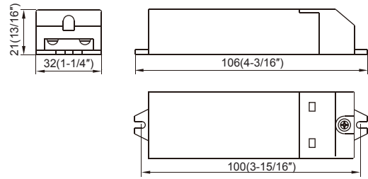
Dimensions: (mm/inches)
