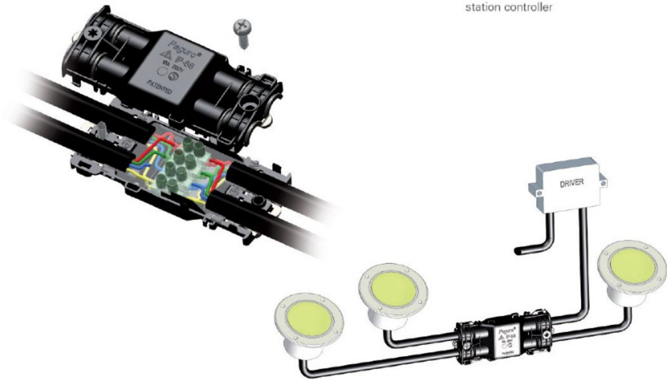
Sketch 2: 3 LED RGB spotlights (cavo with 4 conductors) parallel connected to RGB station controller
